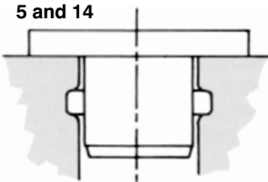
Figure 7: Groove in piston
