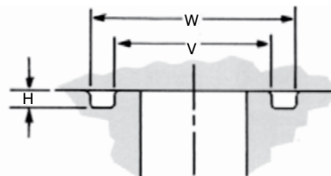
Figure 12: Triangular groove
