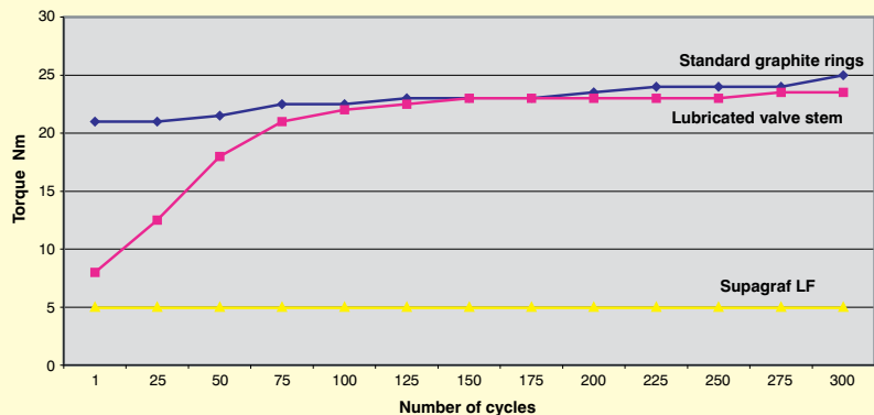
VALVE STEM TORQUE
